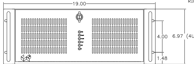
FRONT VIEW - DOOR CLOSED
